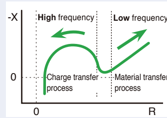
Cole-Cole plot loci and measurement frequency
