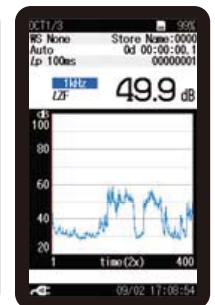
Measurement screen (Level-Time graph)
